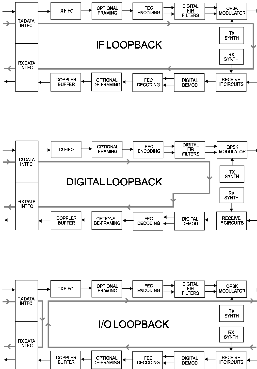
Figure 6-2. Loopback Modes
