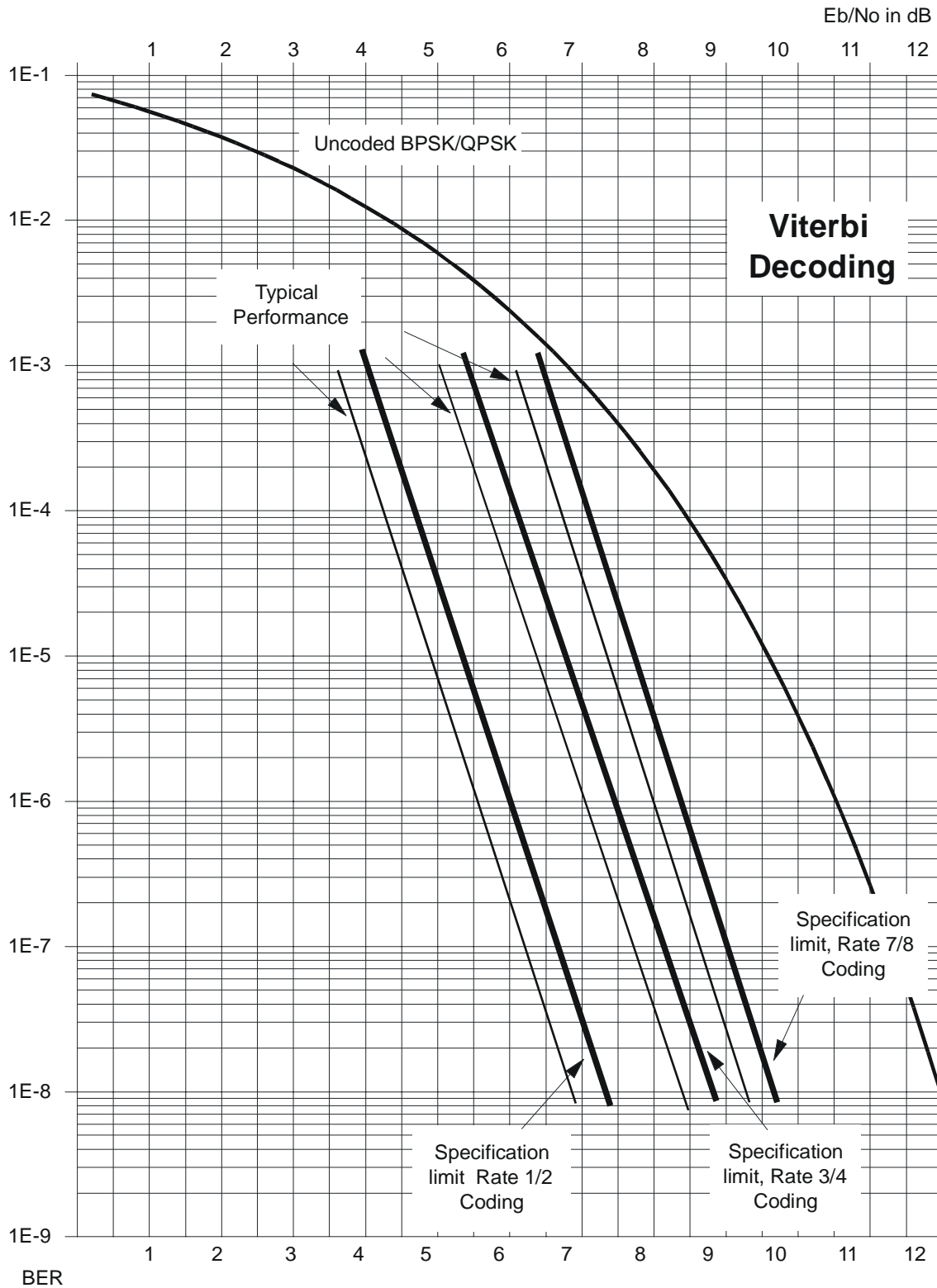
Figure 7-1 Viterbi Decoding
