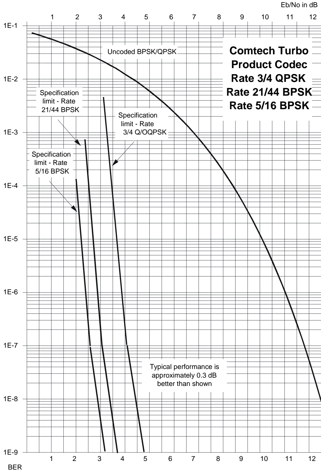
Figure 7-7 Comtech EF Data Turbo Product Codec Rate 3/4 QPSK/OQPSK, Rate 21/44 BPSK, Rate 5/16 BPSK
