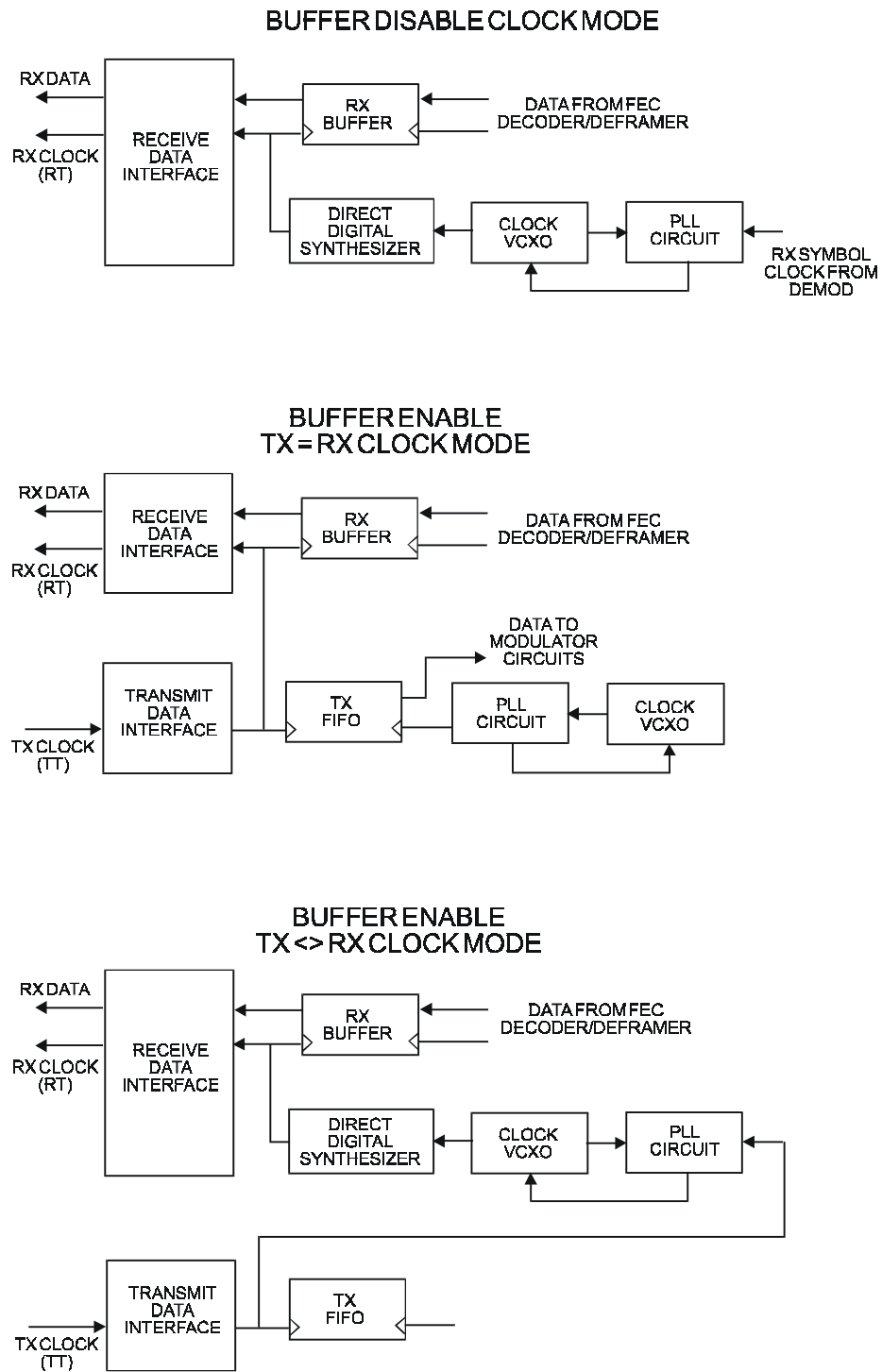
Figure 10-2 RX Clock Modes
