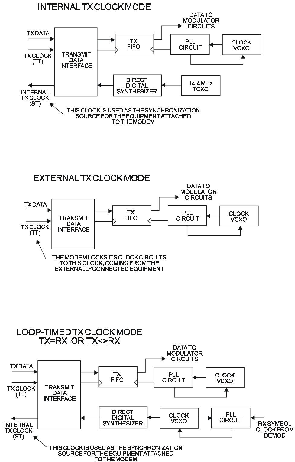
Figure 10-1 Tx Clock Modes
