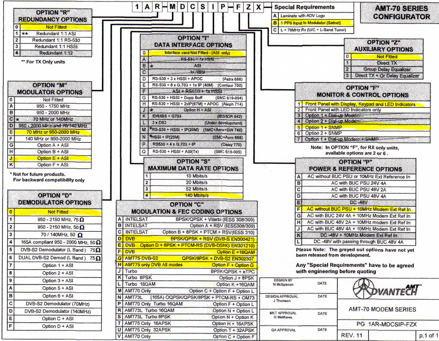
Figure 2: AMT-70 Family: Products Configuration Options
